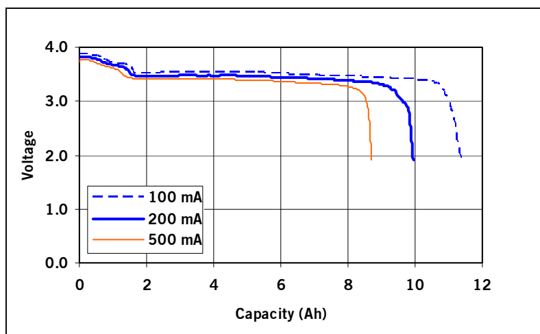
25°C discharge
