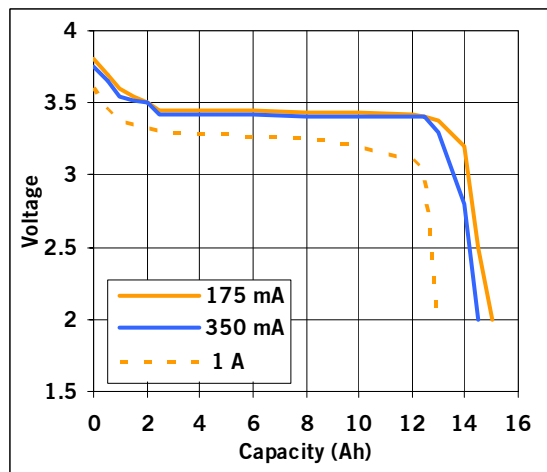
25°C discharge
