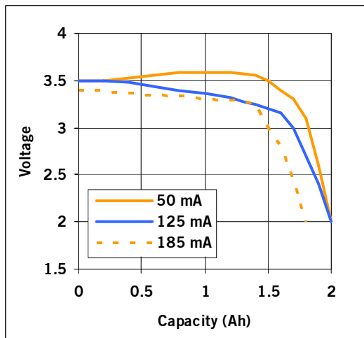
25°C discharge
