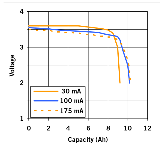
125°C discharge
