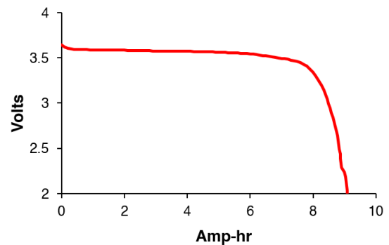
Discharge Curve 100 mA, 150°C
