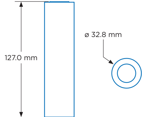
Cell Drawing
