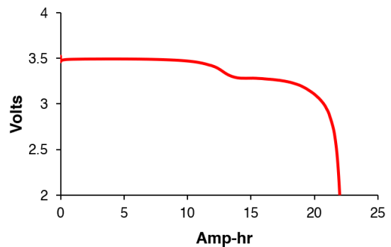
Discharge Curve 500 mA, 120°C
