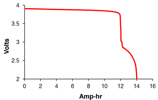
Discharge Curve 50 mA, 120°C
