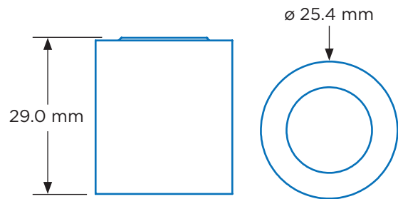
Cell Drawing
