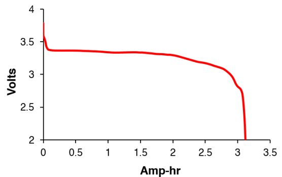
Discharge Curve 75 mA, 23°C
