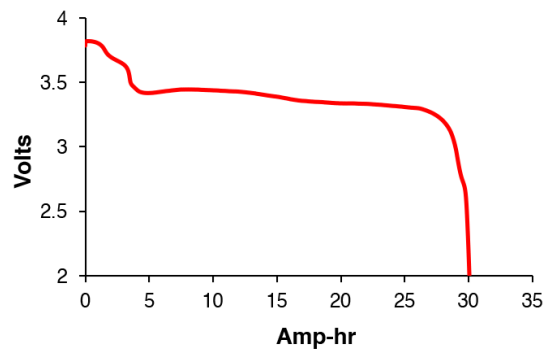
Discharge Curve 350 mA, 23°C
